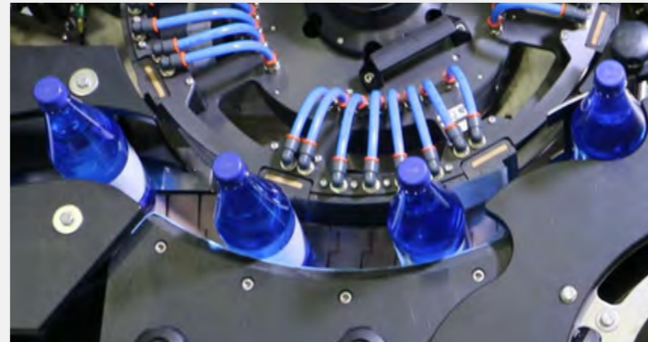
System for rotating bottles
